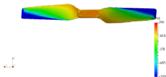
Figure 8. The pressure distribution at the top surface of the blade for the original propeller
