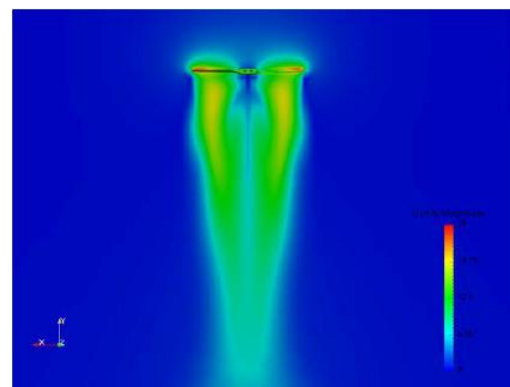
Figure 11. The velocity contours of the cross sectional and surface view for the original propeller
