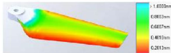
Figure 3. Thickness distribution on 3D model of original propeller.
