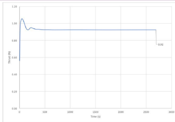
Figure 6. The thrust variation versus simulation time with fine mesh for the original propeller model
