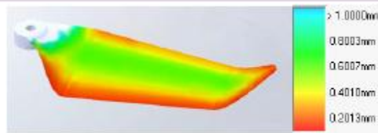
Figure 5. Thickness distribution on propeller with new design.
