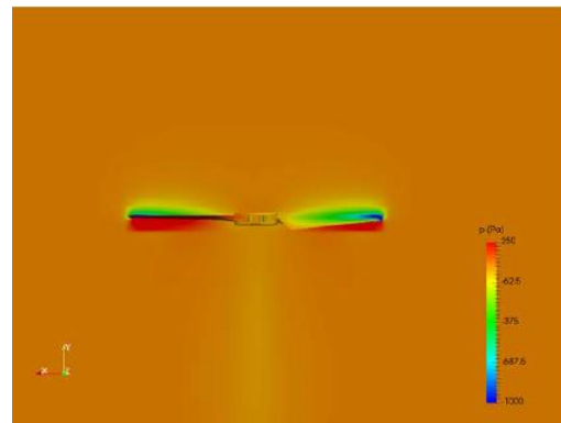
Figure 10. The pressure distribution in the cross sectional and surface view for the original propeller
