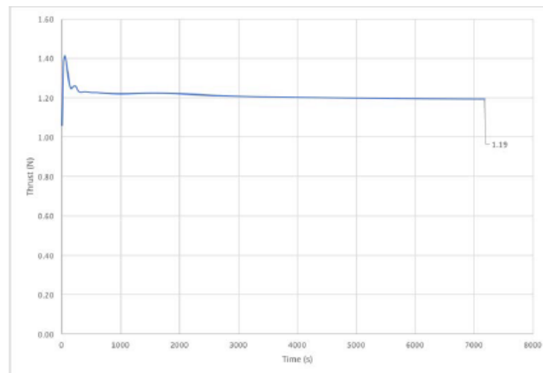
Figure 7. The thrust variation versus simulation time with fine mesh for the winglet propeller
